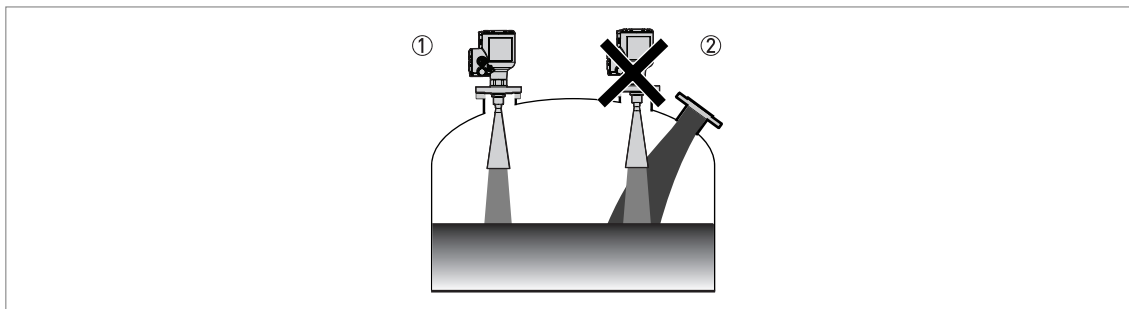
Figure 3-5: Product inlets
