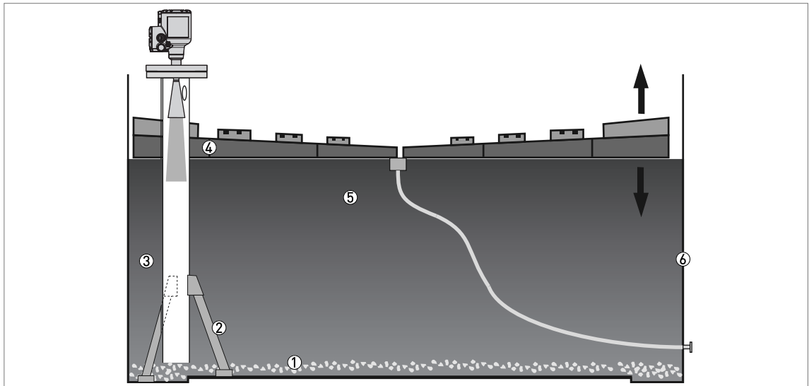
Figure 3-11: Floating roofs
