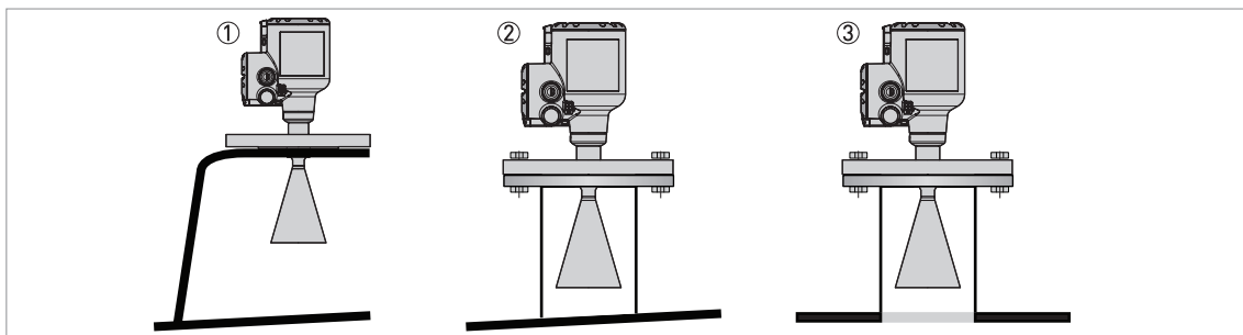
Figure 3-8: Device installation on tanks made of a non-conductive material
