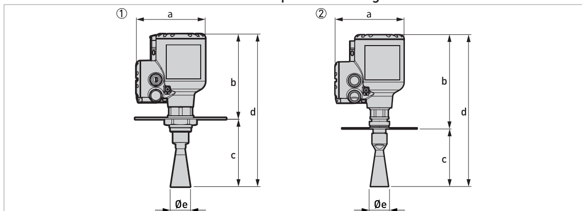
Figure 2-11: Metallic Horn antennas with low-pressure flange connections
